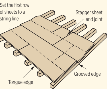
Figure 3. Double Layer Layout
