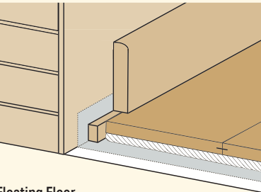
Floating Floor
