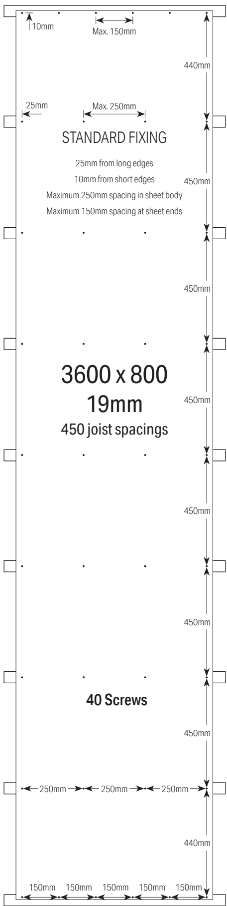
Figure 3. Fixing plan
